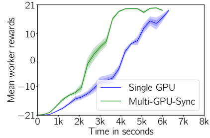
Figure 8. RLgraph synchronous multi-GPU device strategy
