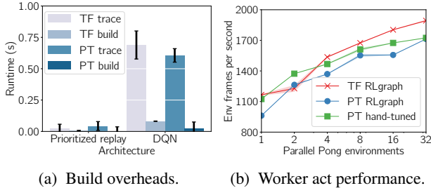
Figure 5. TensorFlow and PyTorch backend comparison.
