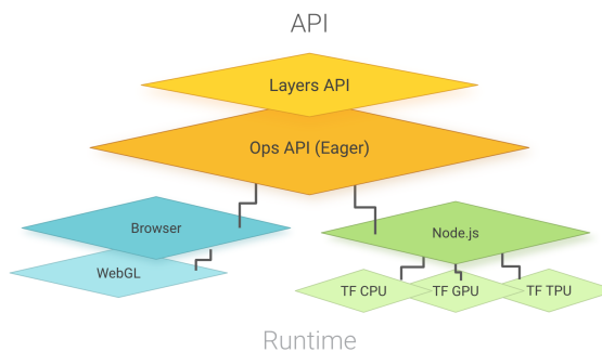
Figure 1. Overview of the TensorFlow.js architecture
